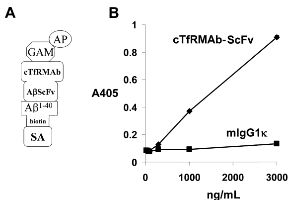
Figure 6. (A) The ELISA used to measure cTfRMAB-ScFv binding to the Aβ 1-40 employs a complex of streptavidin (SA) and N -biotinyl Aβ 1-40 as the capture reagent and a goat anti-mouse (GAM) conjugate of alkaline phosphatase (AP) as the detector reagent. (B) Binding of the cTfRMAB-ScFv fusion protein to the Aβ 1-40 is linear, whereas there is no binding to the Aβ 1-40 of mouse (m) IgG1κ.
