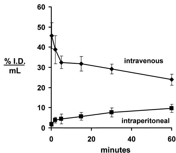
Figure 7. Plasma concentration, expressed as % of injected dose (ID)/mL, of the [ 125 I]-cTfRMAB-ScFv fusion protein after either intravenous or intraperitoneal injection in the mouse. Data are mean ± SE ( n = 3 mice/point).
