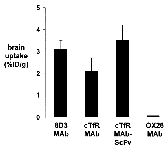
Figure 8. Brain uptake, expressed as % of injected dose (ID)/g brain, for the cTfRMAb-ScFv fusion protein, in comparison with the brain uptake values for the rat 8D3 MAb against the mouse TfR, the mouse OX26 MAb against the rat TfR, and the cTfRMAb reported previously. 4,5 Data are mean ± SE ( n = 3 mice).
