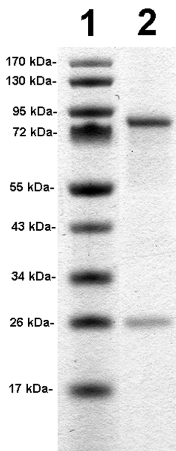
Figure 3. Reducing SDS–PAGE of molecular weight standards (lane 1) and the cTfRMAB-ScFv fusion protein (lane 2). The size of the heavy chain is about 85 kDa, and the size of the light chain is about 26 kDa.
