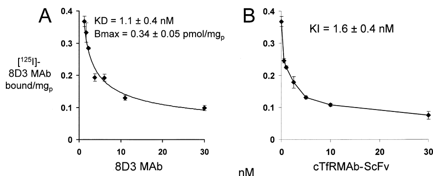
Figure 5. Radio-receptor assay of the mouse TfR uses mouse fibroblasts as the source of the mouse TfR and [ 125 I]-8D3 as the binding ligand. Binding is displaced by unlabeled 8D3 MAb (A) or the cTfRMAB-ScFv fusion protein (B) at concentrations up to 30 nM. The KD of 8D3 self-inhibition and the KI of cTfRMAB-ScFv cross-inhibition were computed by nonlinear regression analysis.
